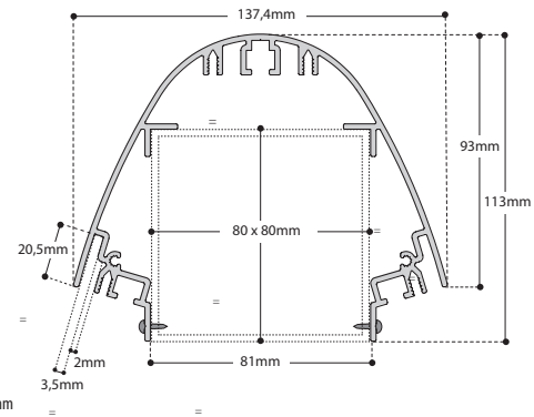
Aluminium or steel profile 80 x 80 x 4mm Tube de fondation 80 x 80 x 4mm
